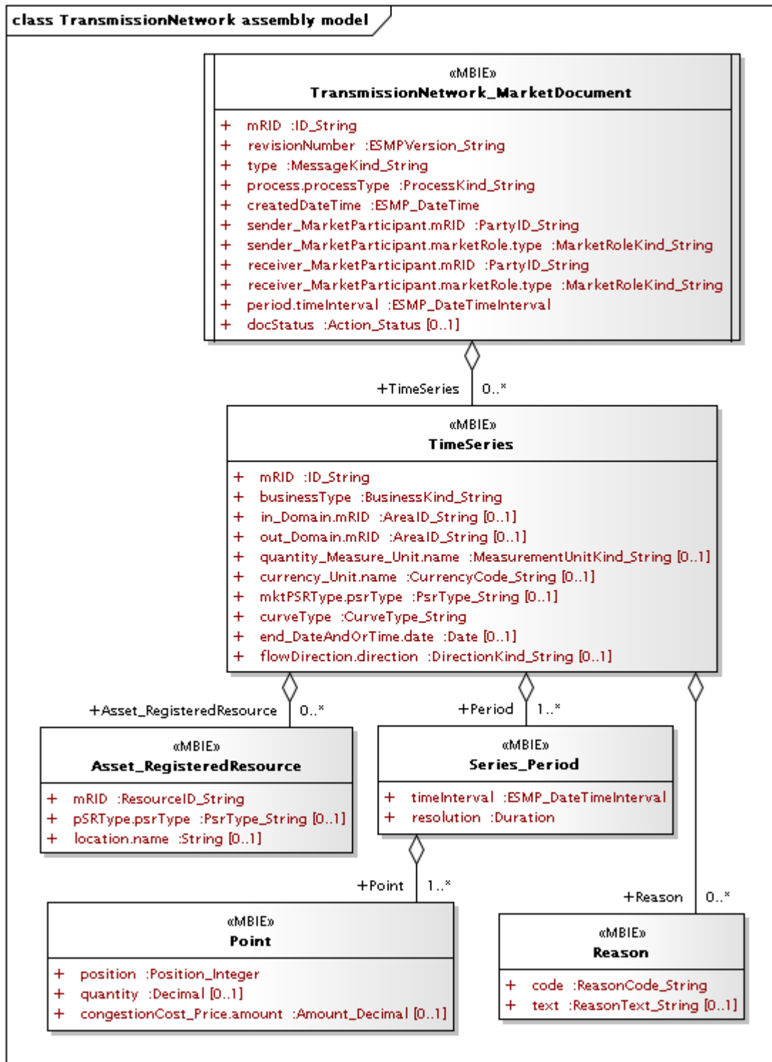
Figure 12 – TransmissionNetwork assembly model
