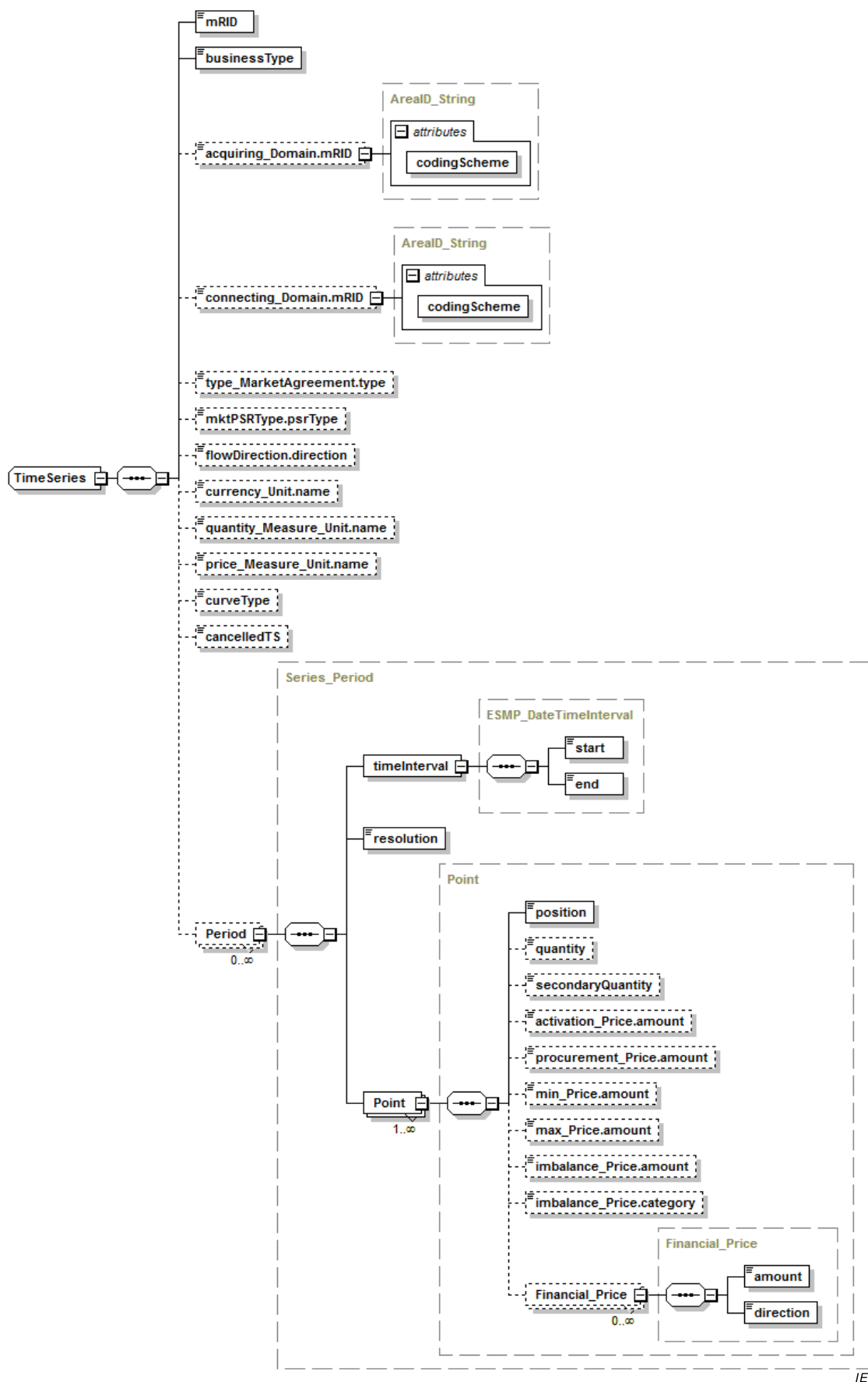
Figure 20 – Structure de schéma XML Balancing_MarketDocument – 2/2
