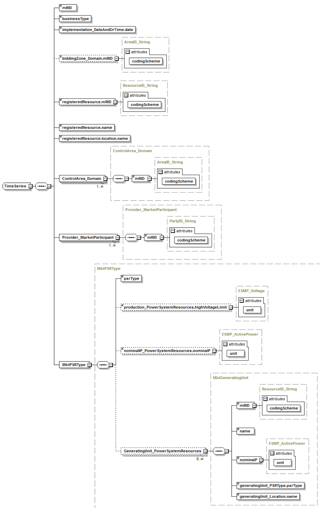
Figure 24 – Structure de schéma XML Configuration_MarketDocument – 2/2
