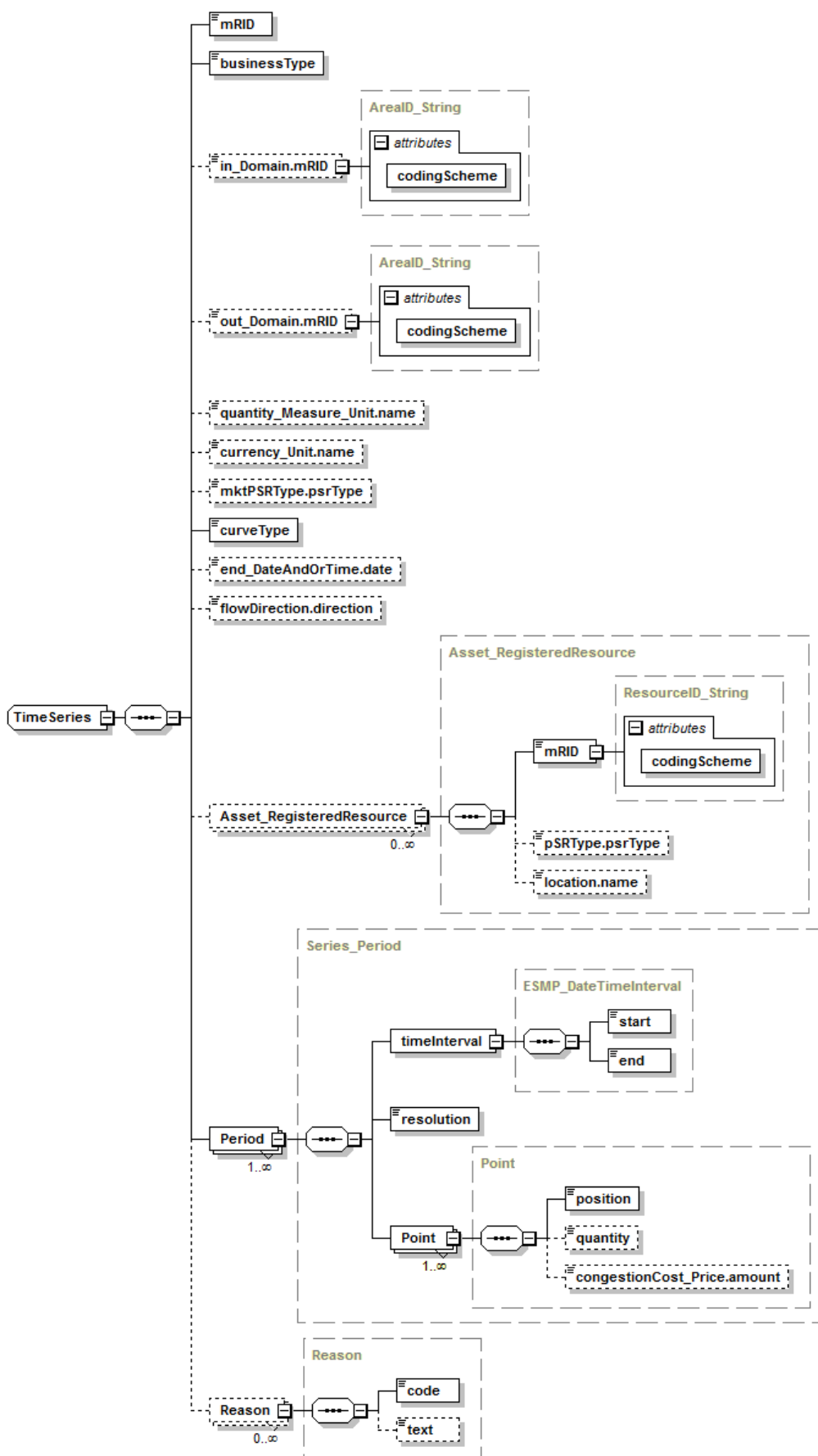
Figure 22 – Structure de schéma XML TransmissionNetwork_MarketDocument – 2/2
