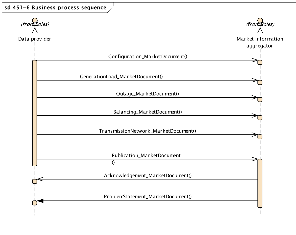
Figure 4 – Sequence diagram of the information flows
