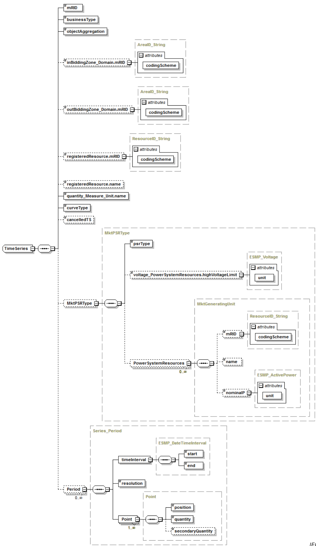
Figure 16 – Structure de schéma XML GenerationLoad_MarketDocument – 2/2
