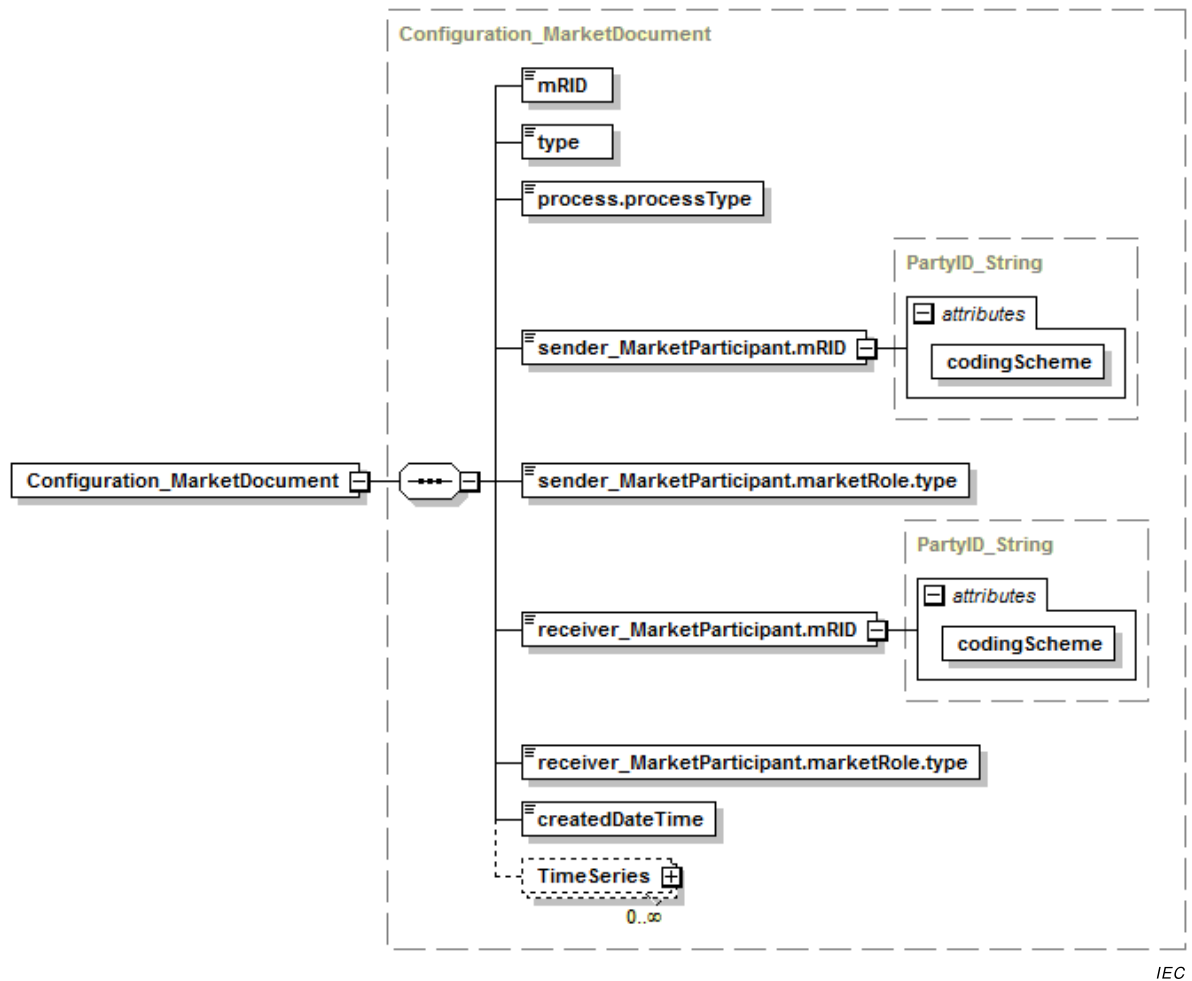
Figure 23 – Configuration_MarketDocument XML schema structure – 1/2
