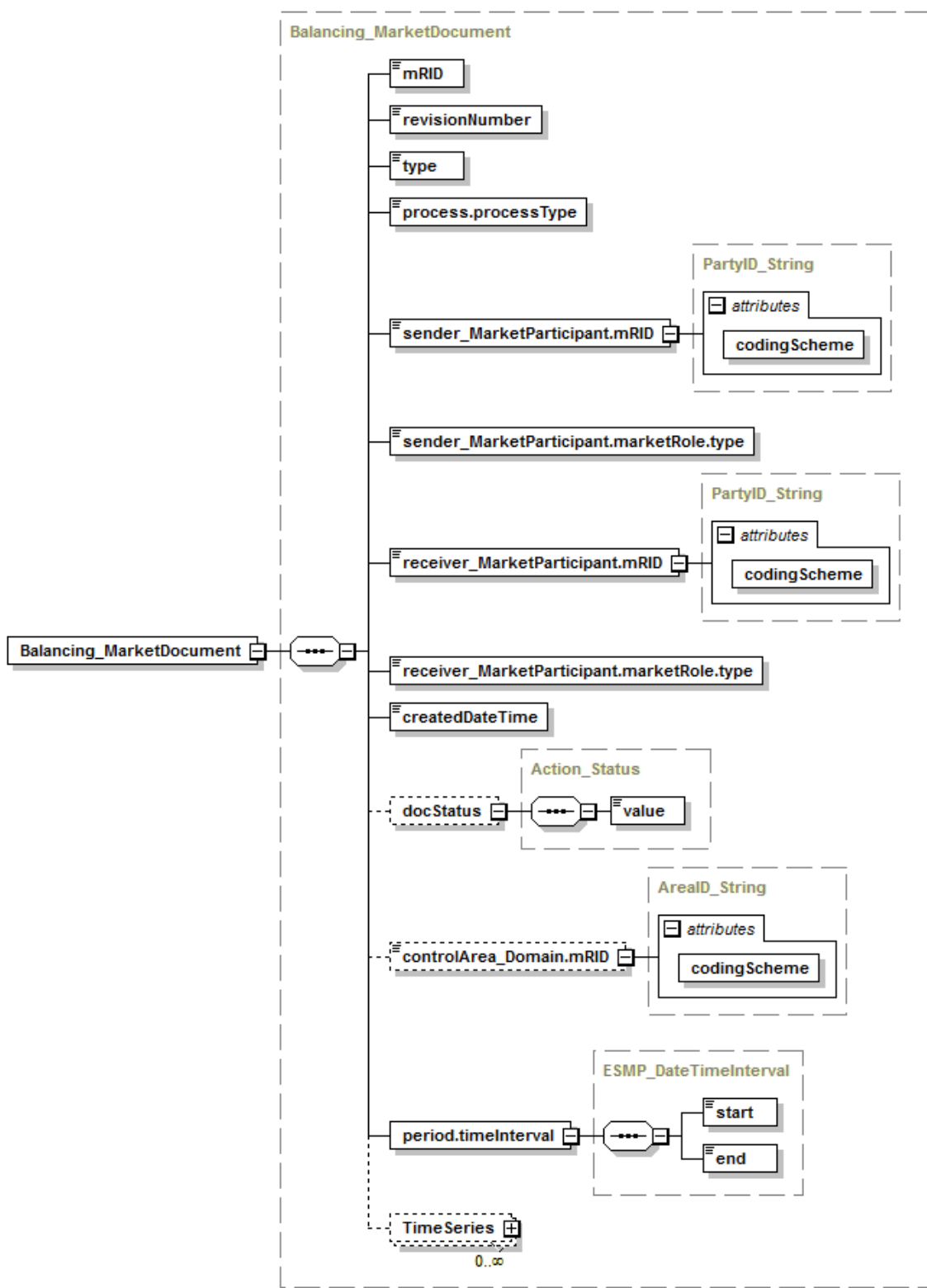
Figure 19 – Structure de schéma XML Balancing_MarketDocument – 1/2
