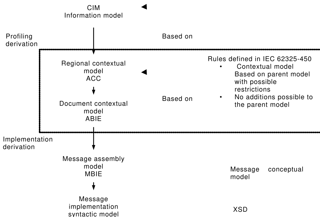
Figure 1 – IEC 62325-450 modelling framework
